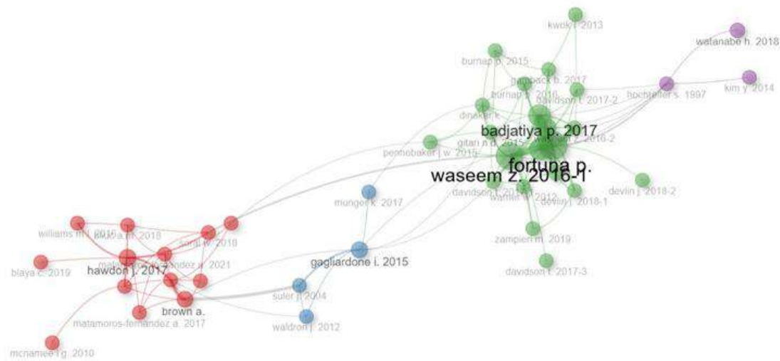
Fig. 10 Co-Citation Network
