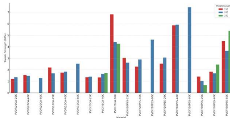
Figure 8: Tensile Strength by Material and Thickness
