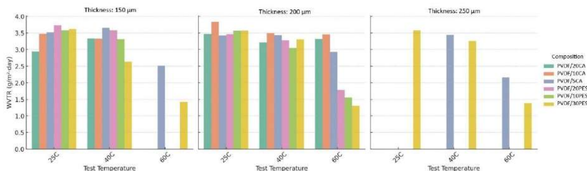
Figure 10: MVTR Comparison by Composition and Temperature
