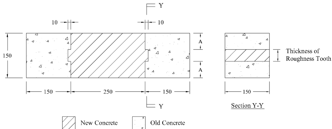
Figure 1. Typical Detailing of Numerical Specimens
