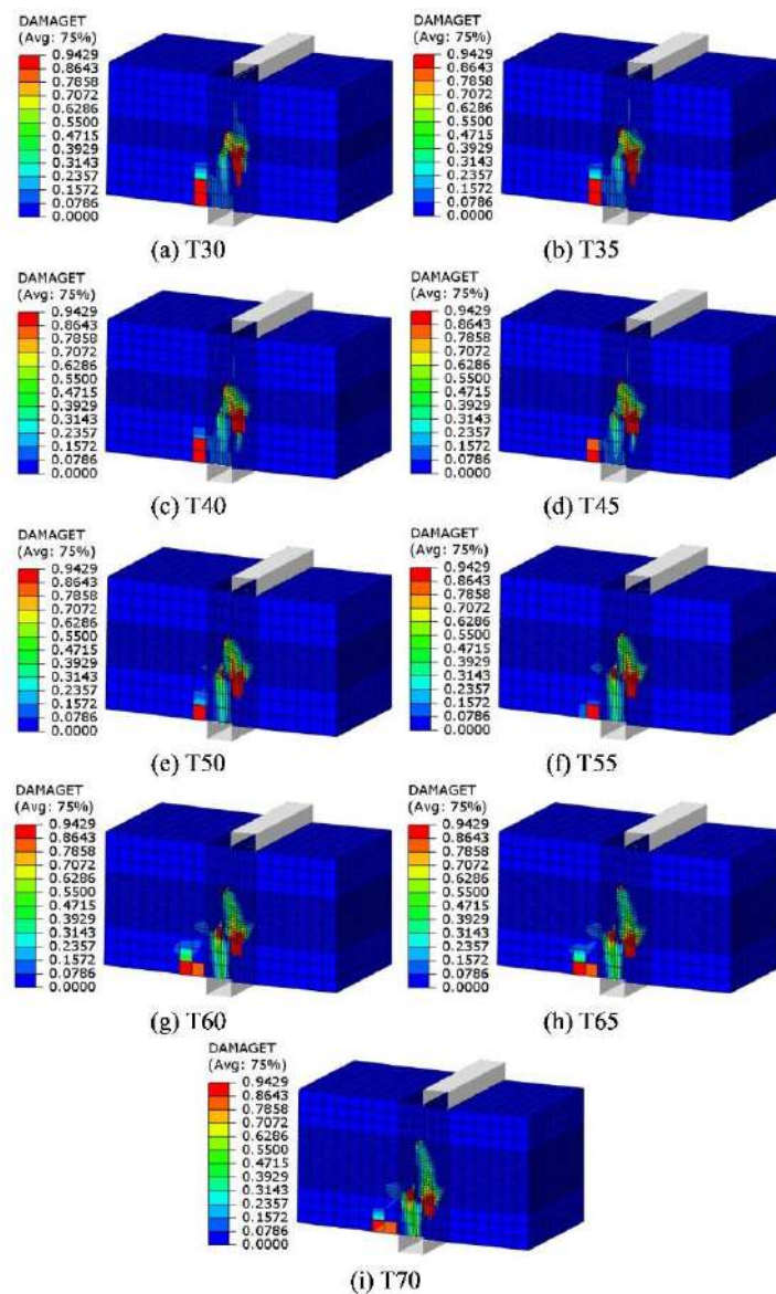
Figure 12. Damaget Contours for All Numerical Specimens
