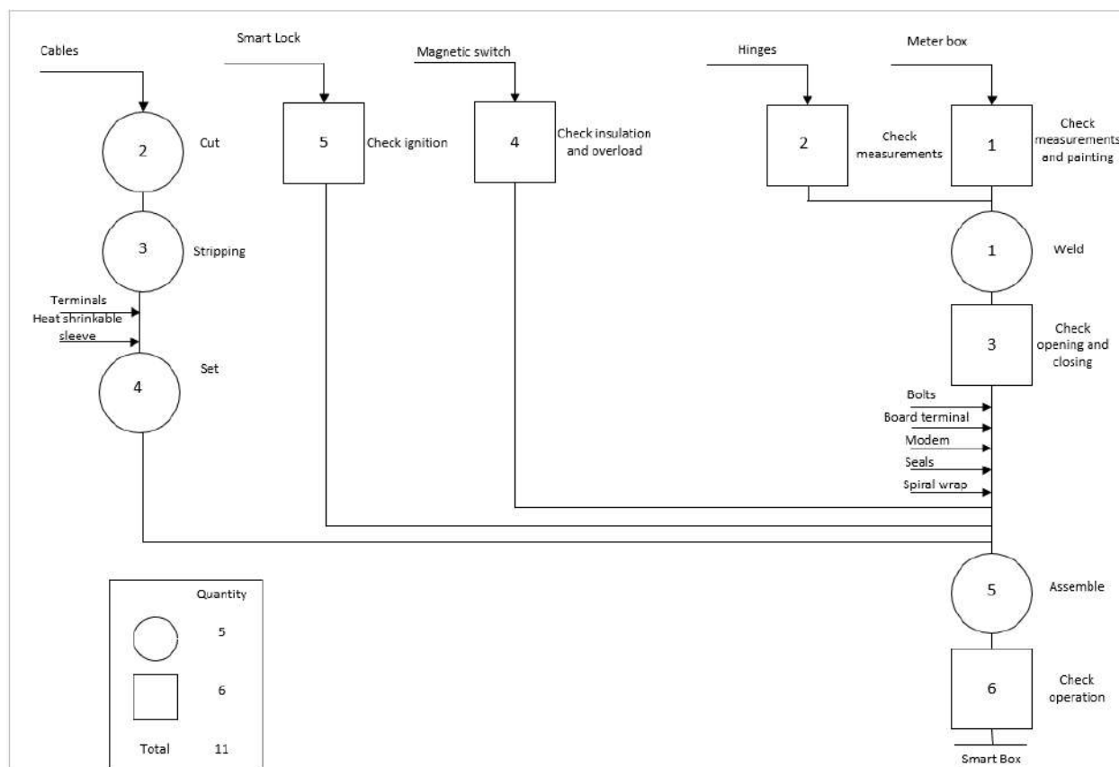
Figure 1. Operation Process Chart (OPC) of the Smart Box Production Process
