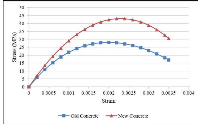
Figure 3. Uniaxial Stress-Strain Curves under Compression
