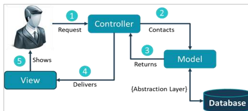
Figure 1. Block diagram of the developed database content manager's architecture
