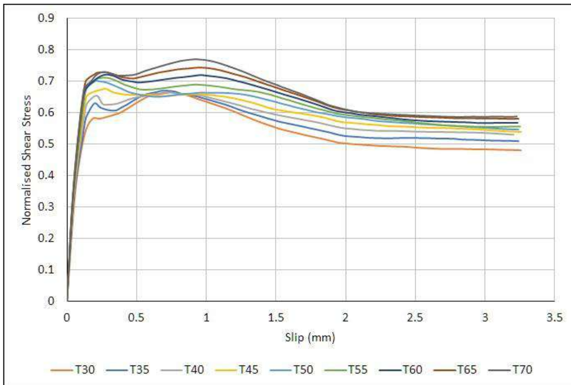
Figure 9. Normalised Shear Stress-Slip Curves for All Numerical Specimens
