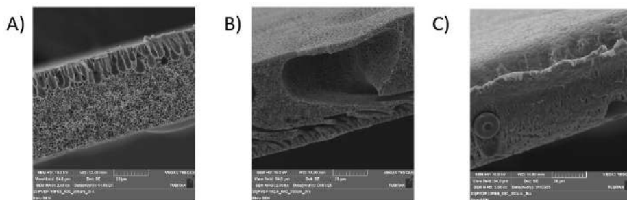
Figure 11: SEM images A) PV/PES-10, B) PV/CA-10 C) PV/PES-05
