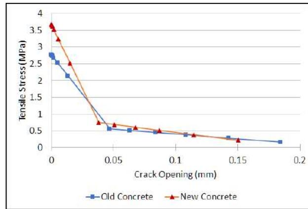
Figure 6. Concrete Tensile Stress versus Crack Opening Graph
