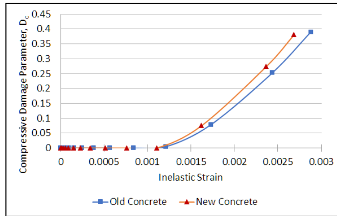
Figure 5. Concrete Compressive Damage Parameter against Inelastic Strain Graph
