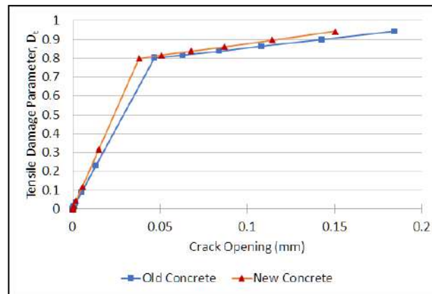
Figure 7. Concrete Tensile Damage Parameter against Crack Opening Graph
