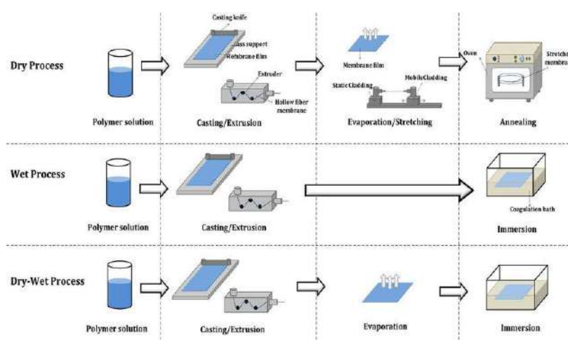
Figure 6: Dry, Wet and Dry/Wet Phase Inversion Processes
