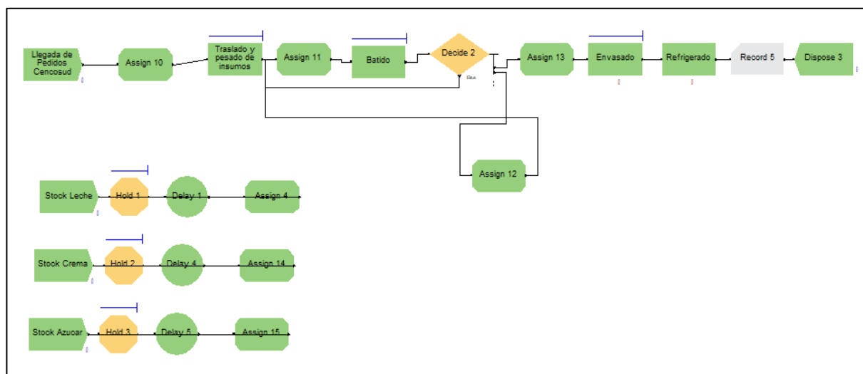
Figure 1. Arena model of the company's ideal inventory and production process
