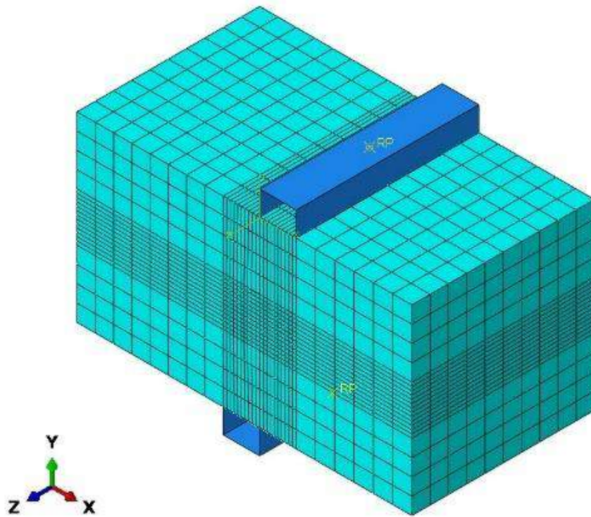
Figure 8. Meshing of Model
