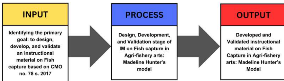
Figure 1. IPO Model
