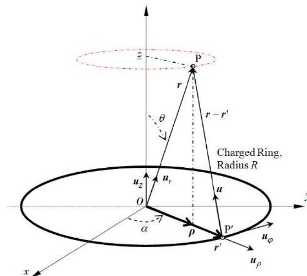
Figure 1. A ring of radius R lies on the xy plane. The field point P has cylindrical coordinates (\rho, z) .
