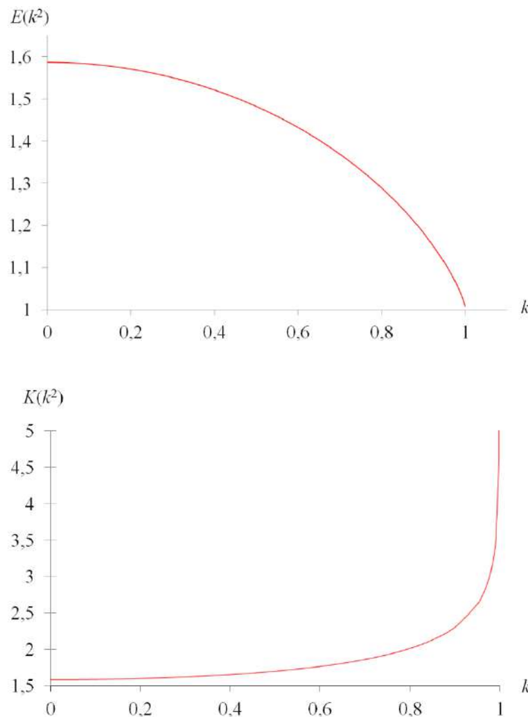
Figure 3. Complete elliptic integrals of the first and second kinds as functions of the Modulus k .
