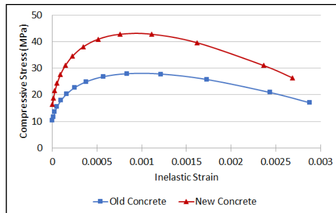
Figure 4. Concrete Compressive Stress versus Inelastic Strain Graph
