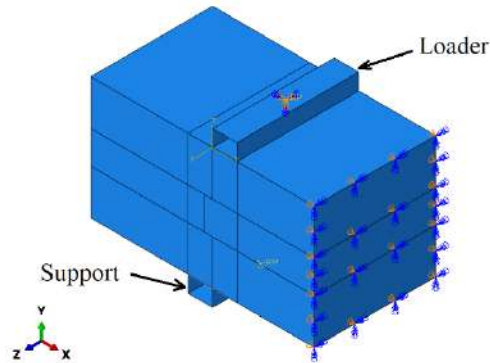
Figure 2. Numerical Specimen Testing Setup
