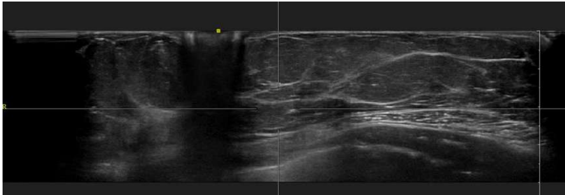
Fig. 3 Retroareolar shadowing.
