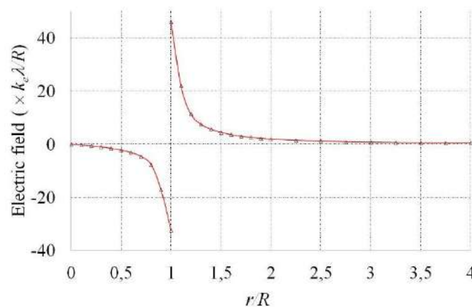
Figure 4. Electric field amplitude in the plane of a uniformly charged ring as a function of the relative radius a=r/R .
