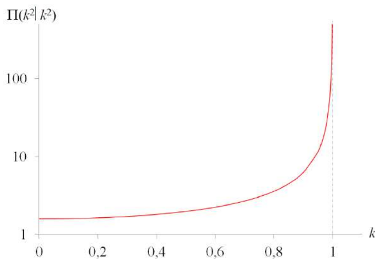
Figure 2. Complete elliptic integral of the third kind \Pi(k^2|k^2) vs. modulus k .
