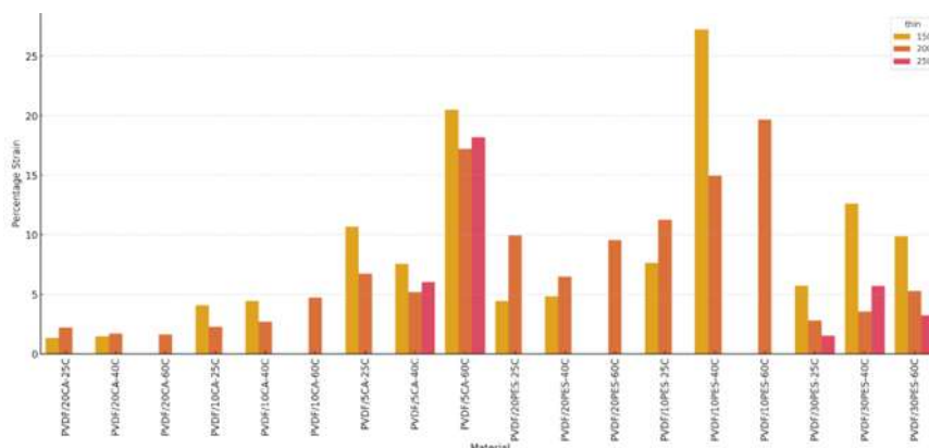
Figure 9: Percentage Strain at Maximum Load By Material and Thickness
