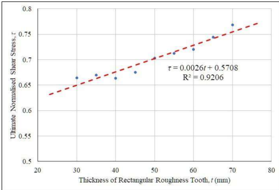
Figure 10. Correlation between Ultimate Normalised Shear Stress with Tooth Thickness
