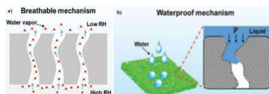
Figure 2: Hydrophobic Microporous Membrane
